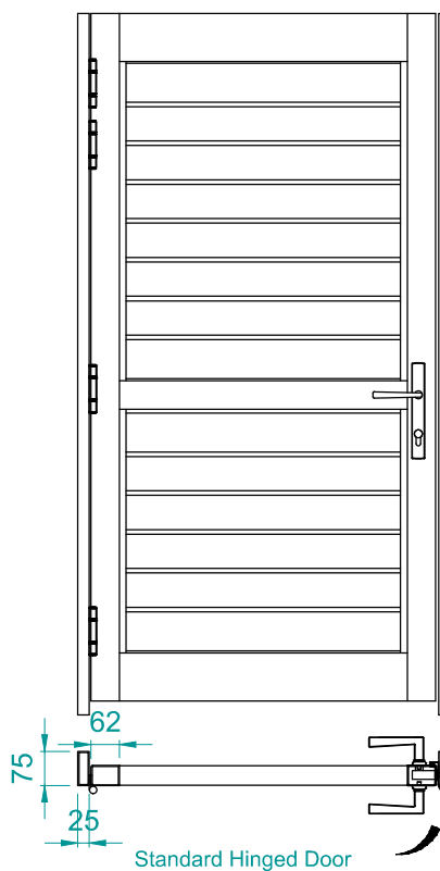
heavy duty hinged door with transom Louvres in closed position.
