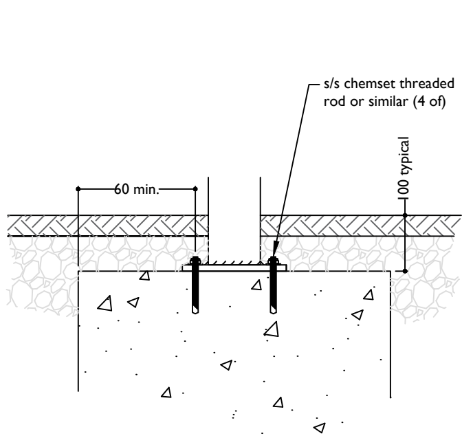
SECTION POST TO CONCRETE FOOTING - RECESSED
